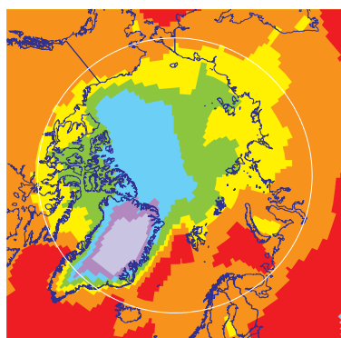
GEOS-Chem model
