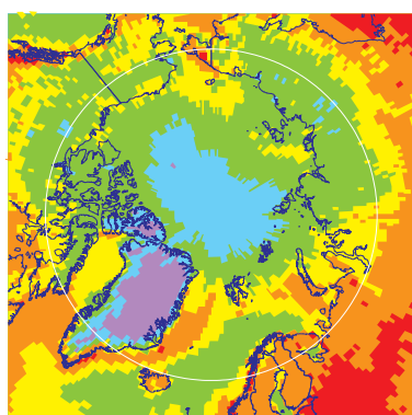
GRAHM model
