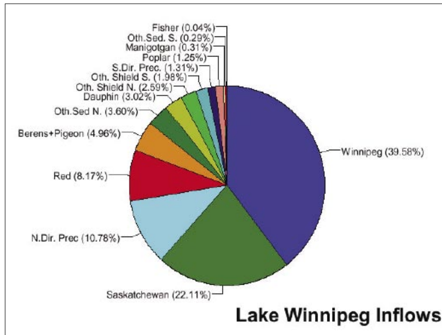
Fig. 5. Relative inflow volume contribution by major rivers to Lake Winnipeg 60
