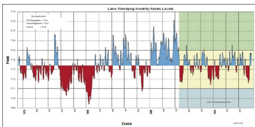
Fig. 7. Lake Winnipeg monthly mean water levels (1912 – 2004) 66
