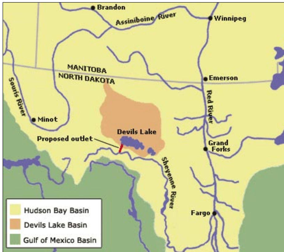
Fig. 32 Location of Devils Lake Basin within the Hudson Bay Drainage Basin 269 . Devils Lake is the larger of the two lakes within the Basin, Stump Lake is the smaller
